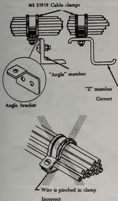
FIGURE 4-98. Mounting cable clamp to structure.
